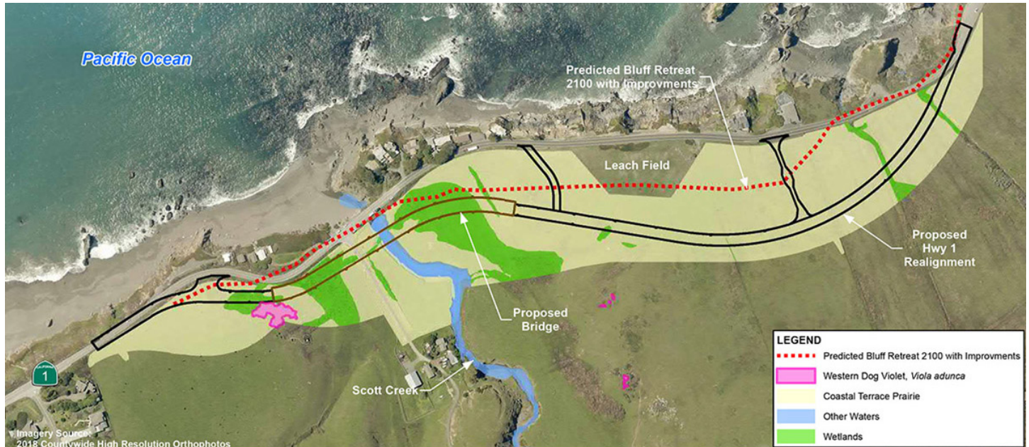
Image 10. Realignment diagram of Highway 1 near Gleason Beach in Sonoma County. Photo by Caltrans .
