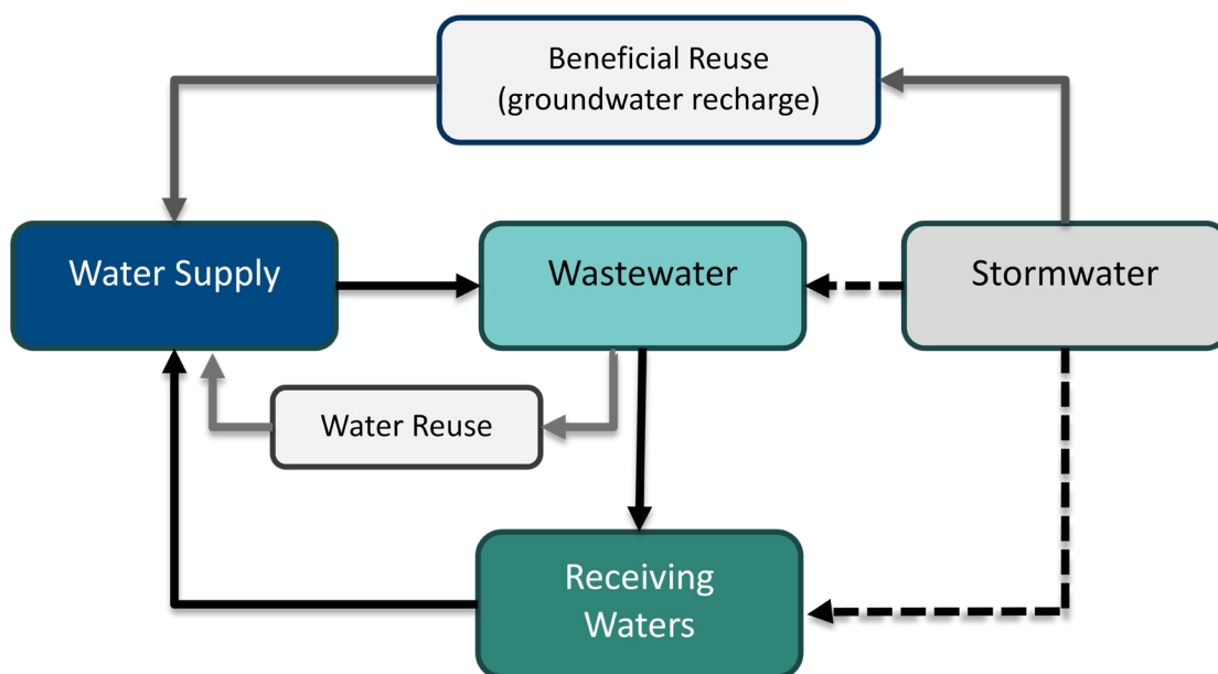
Figure 4. Conceptual diagram of holistic approach to water management using water supply, wastewater, and stormwater systems. Dashed arrows indicate where BMPs can reduce flows and gray arrows indicate water recharge or reuse. (Adapted from EPA 2012 Water Reuse Guidelines)
