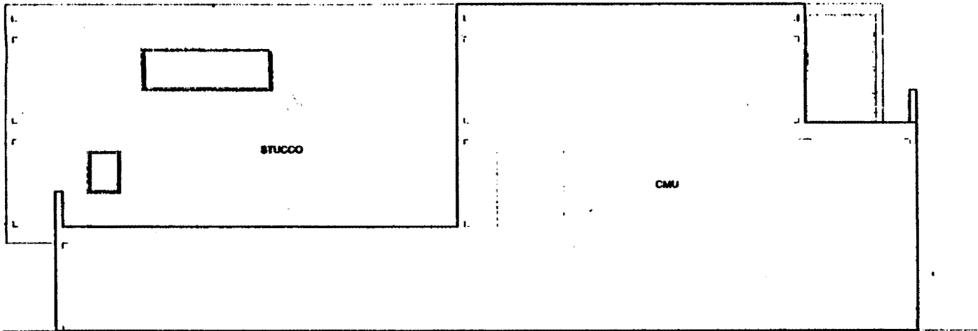
EAST ELEVATION
