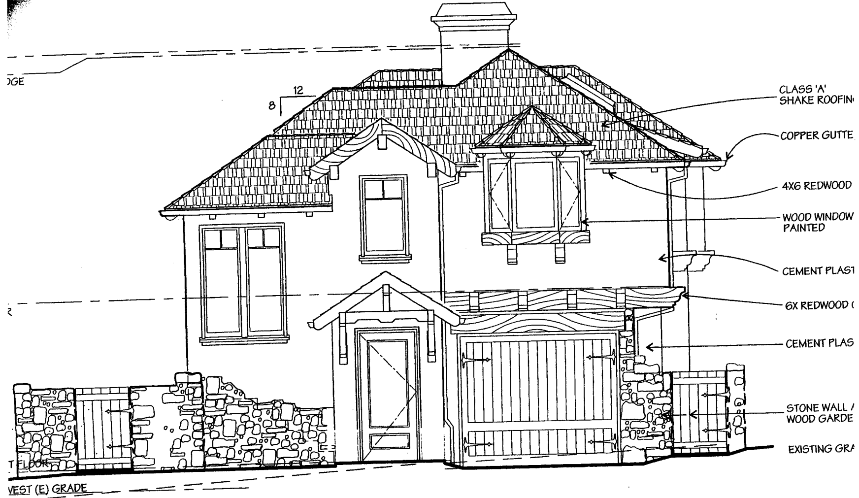
East Elevation
