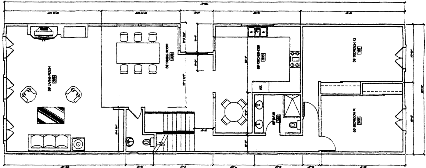
PROPOSED SECOND FLOOR PLAN 1770 SQ. FT.
