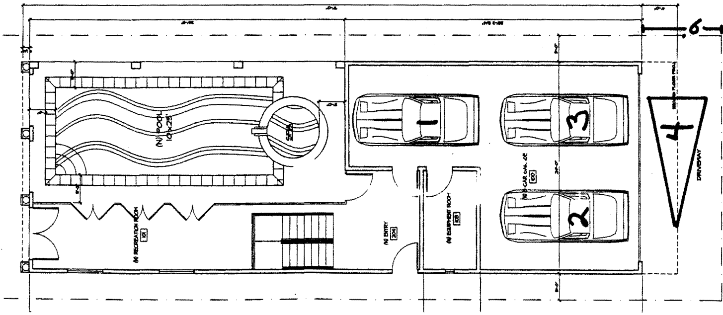
PROPOSED FIRST FLOOR PLAN 860 SQ. FT.
