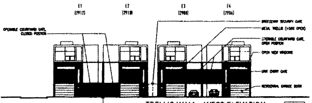
TRELLIS WALL: WEST ELEVATION (VIEW FROM LAFAYETTE STREET)
