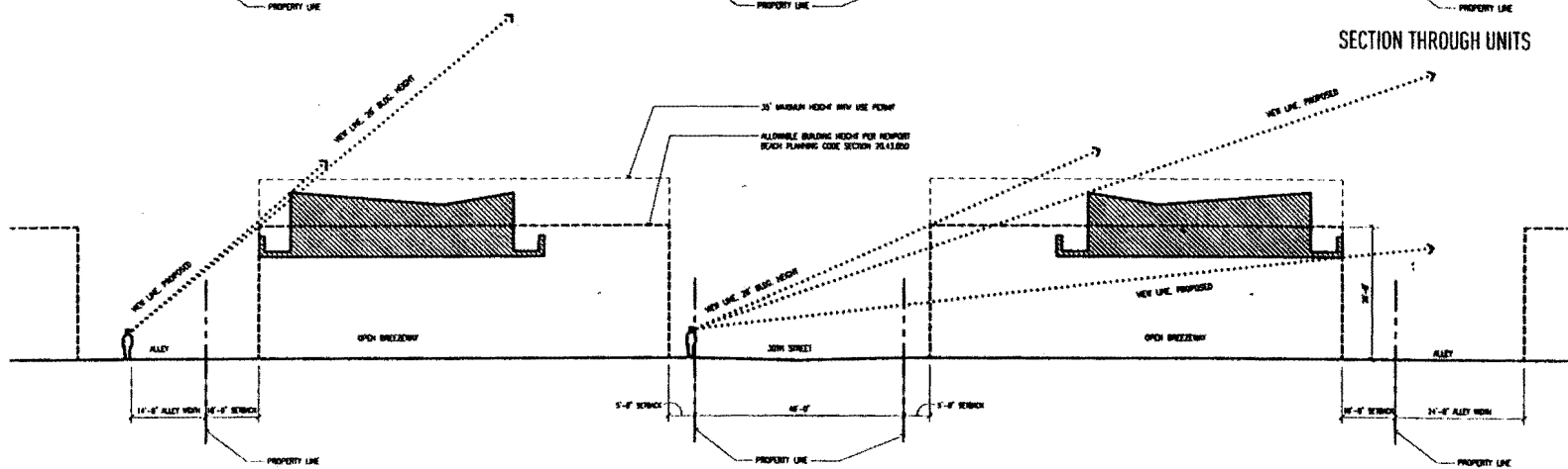
SECTION THROUGH BREEZEWAY
