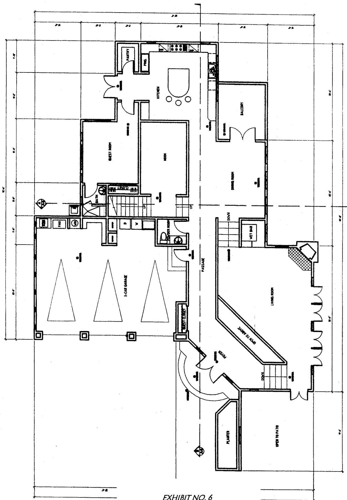
EXHIBIT NO. 6 APP. NO. 4-03-040 LOWER FLOOR PLAN
