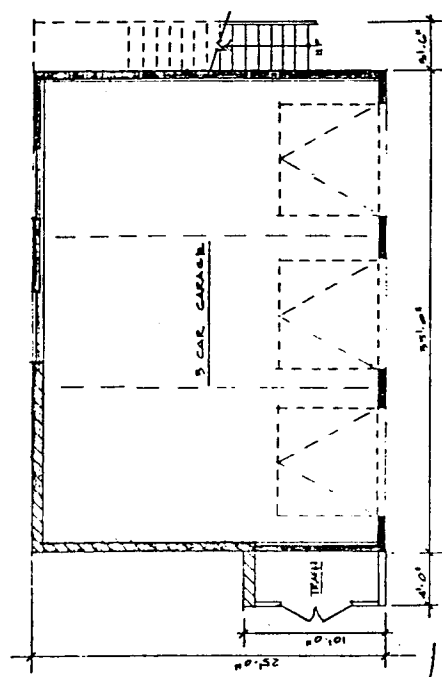
FIRST FLOOR PLAN - GARAGE - 875 S.F. SCALE 1/8" = 1'-0"
