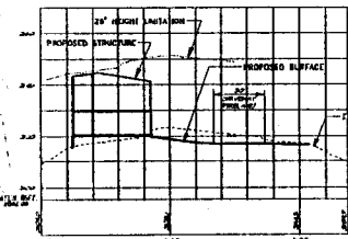
Section "Z"-Z" PROFILE SCALE: 1"=40' VERT. SCALE: 1"=40'
