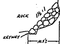
SECTION A-A ROCK REVETMENT SECTION
