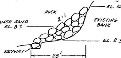
SECTION B-B ROCK REVETMENT SECTION
