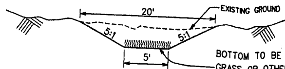
③ 20' GRASSY SWALE
