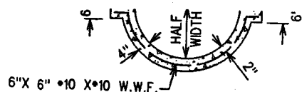
② SEMICIRCULAR DITCH
