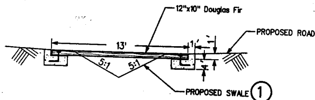
④ SWALE CROSSING
