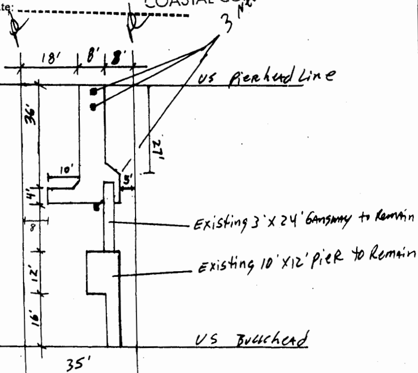
PLAN VIEW 1" = 30'
