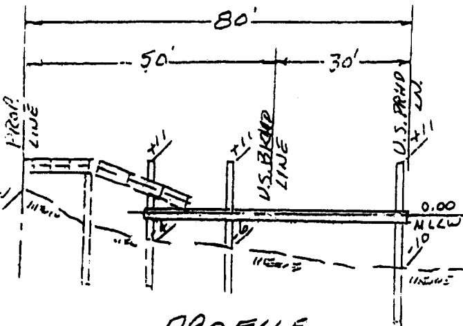
PROFILE 1" = 30'
