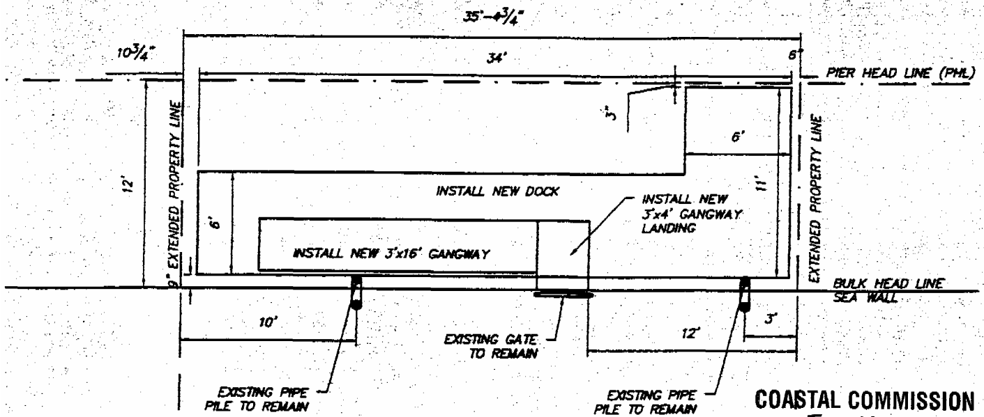
NEW DOCK LAYOUT
