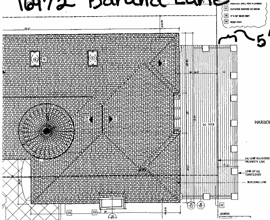
5-08-143 Exhibit B Site Plan/Plan View
