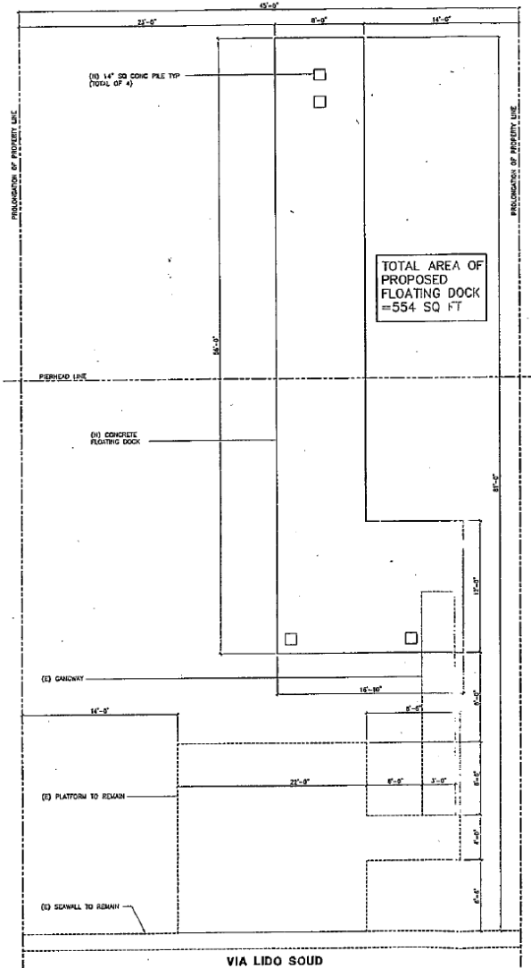
R PROPOSED PLATFORM, DOCK, GANGWAY AND PILING LAYOUT
