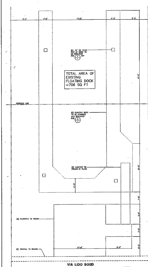
T EXISTING PLATFORM, DOCK, GANGWAY AND PILING LAYOUT
