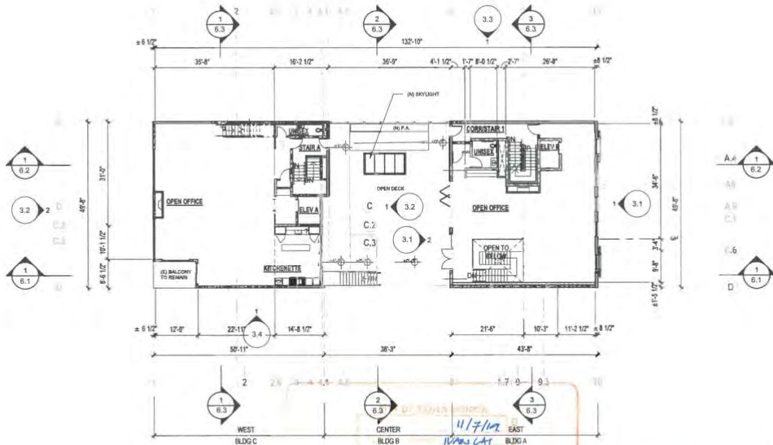
THIRD FLOOR PLAN SCALE: 1/16" = 1'-0"
