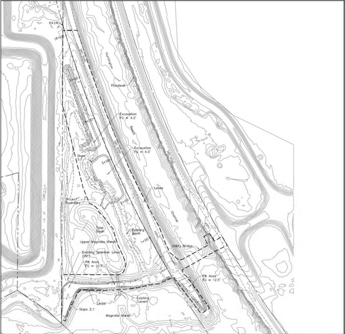
UPPER MAGNOLIA MARSH GRADING PLAN
