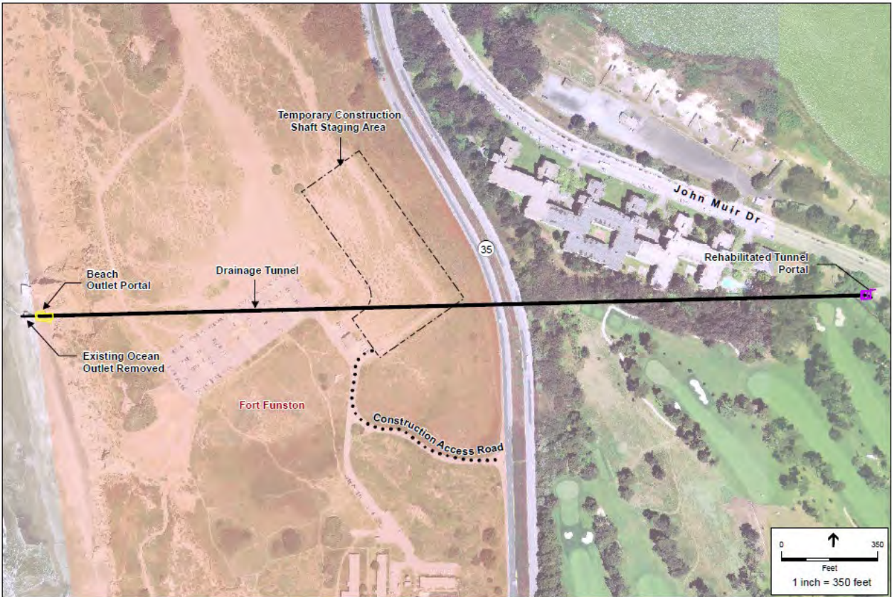
Figure 4: Tunnel and Ocean Outlet project components.
